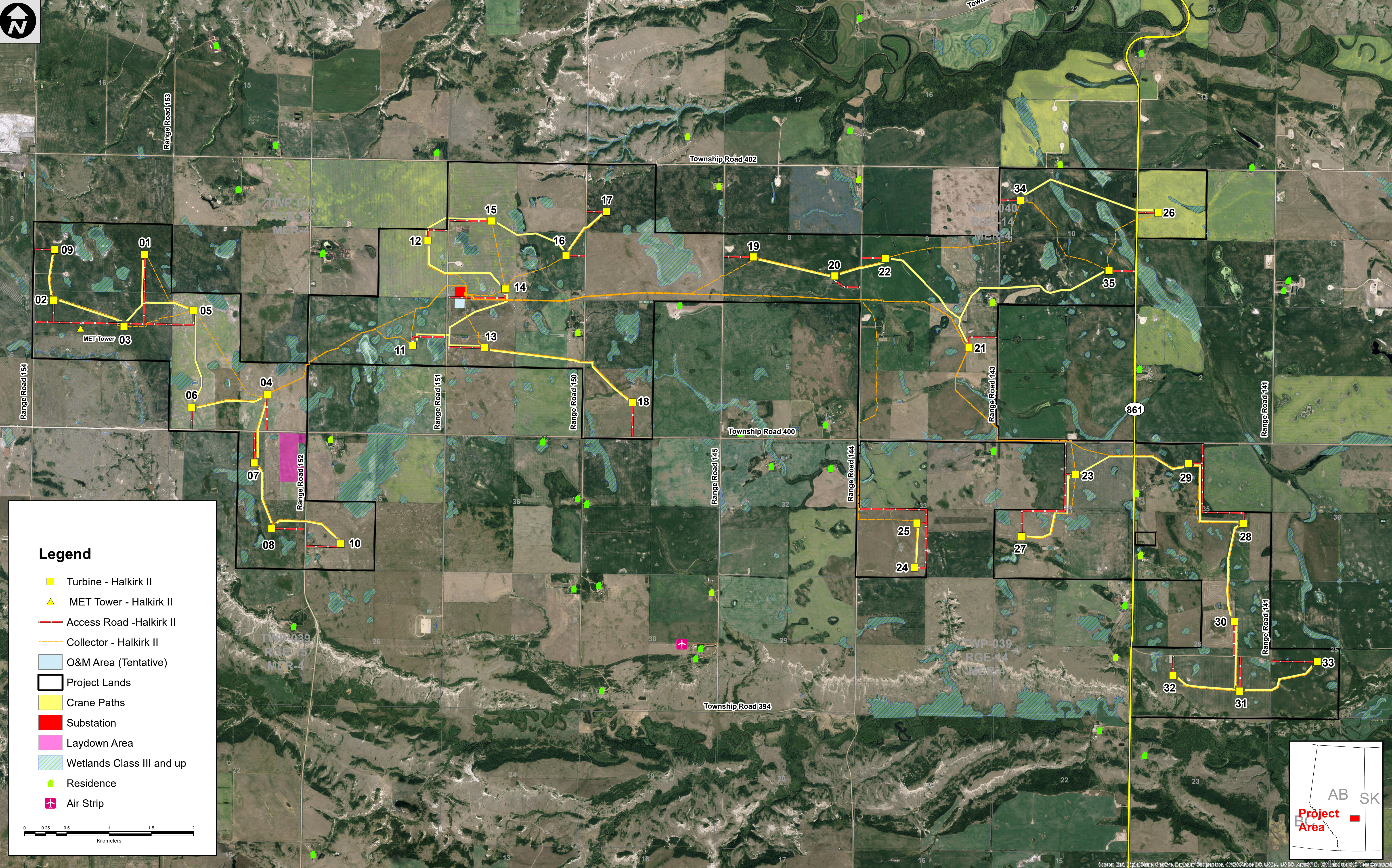
Exhibit A: Halkirk 2 Wind Project Final Design Layout
