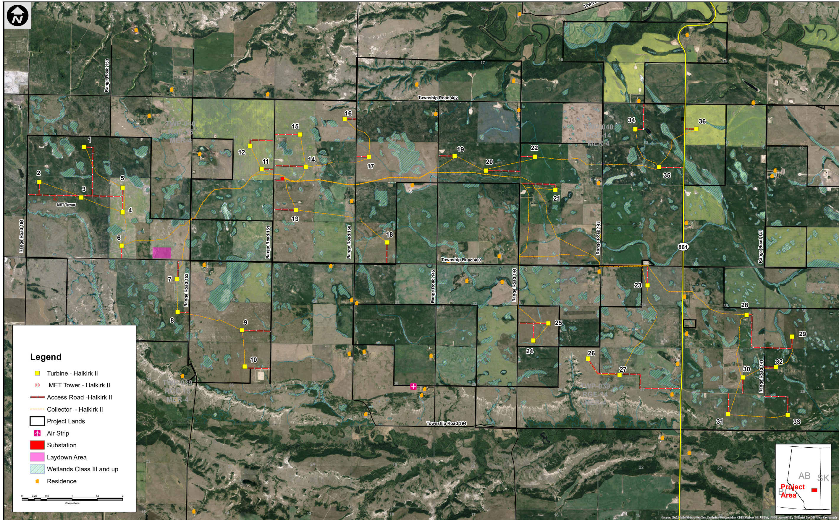
Exhibit A: Halkirk 2 Wind Project Layout
